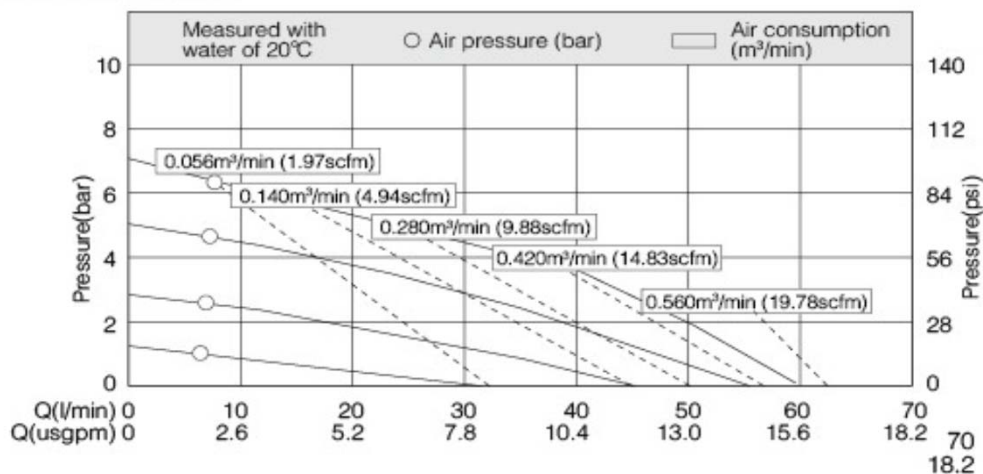
Performance curve
